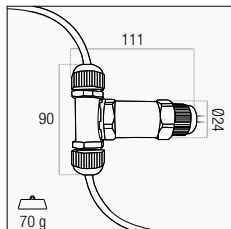
T 3 VIE / T 3 WAY
