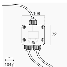
BOX 3 VIE / 3 WAY
