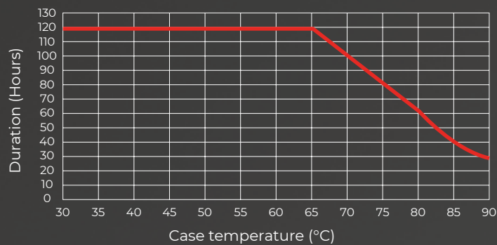
Product life curve
